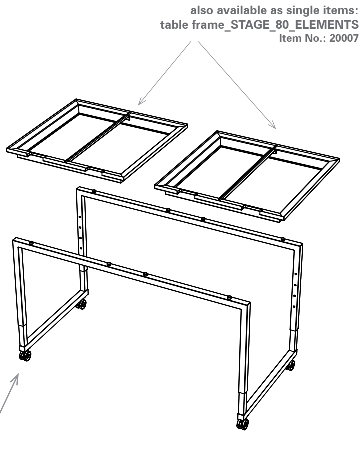
STAGE_80_S_ELEMENTS Item No.: 20101
